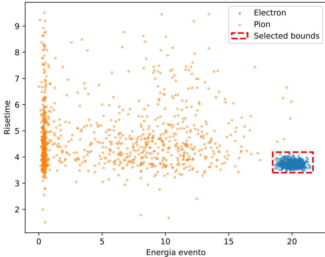
Scatter plot e/pi (all) 20.0GeV
