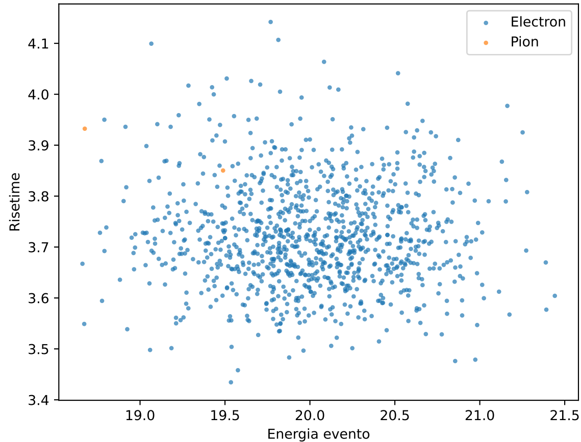
Scatter plot e/pi (cutted) 20.0GeV
